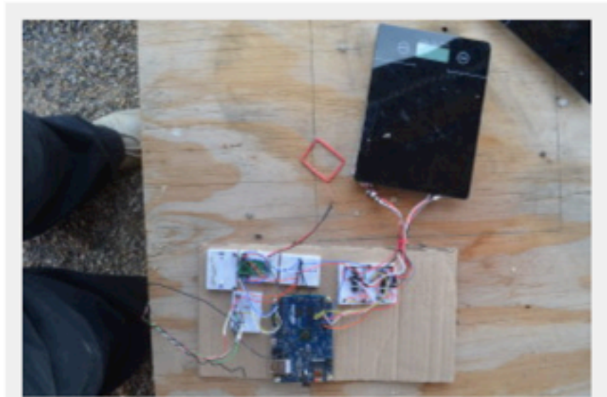
The Galileo, a scale and RFI setup. Nelson details, “The scales have 4 load sensors each. Each load sensor has 3 wires, and is 1/2 of a wheatstone. I joined two load sensors to make 1 wheatstone bridge and connect each wheatstone bridge to an instrumentation amplifier (TI INA125p). I calibrated the voltage output of the amplifiers to known egg weights and hen weights.”
