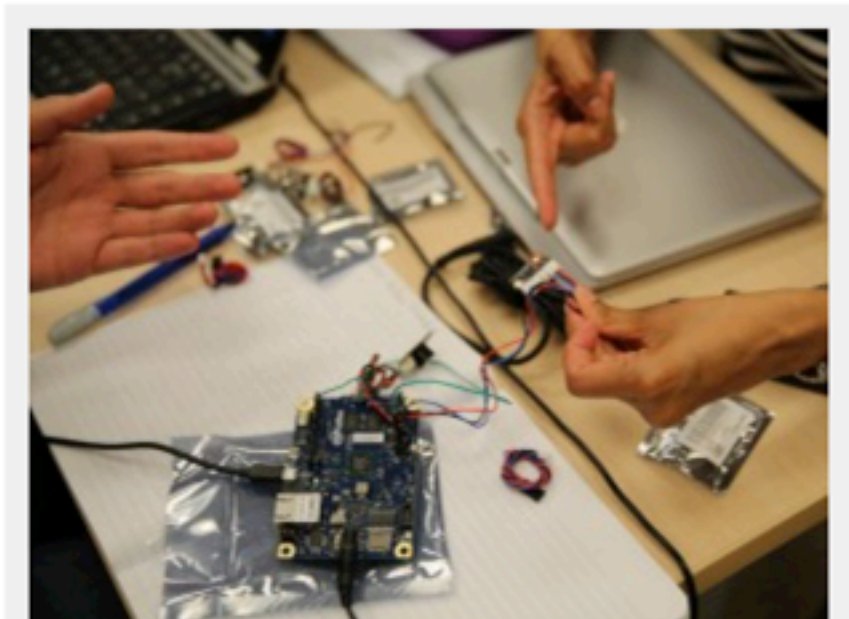
Getting actuators and input sensors to work was core to the Galileo development board wearables workshops, with team members collaborating on the design and technical implementation of the design.
