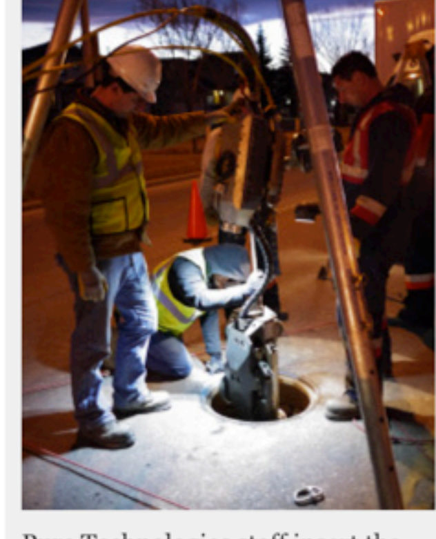
Pure Technologies staff insert the PureRobotics tool into a live pipeline in Calgary, Alberta inspect for structural deterioration. Photo credit: Pure Technologies Ltd.
